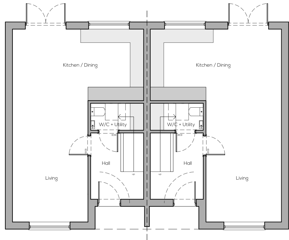
P5 Ground Floor Plans
