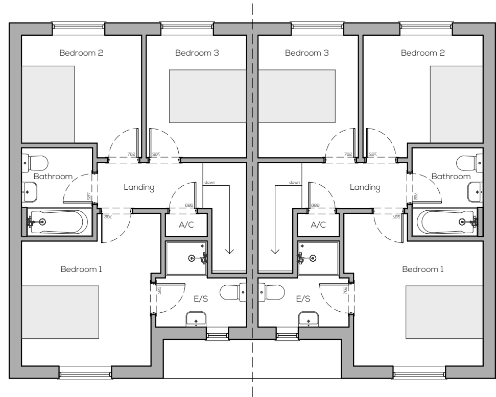
P5 First Floor Plans
