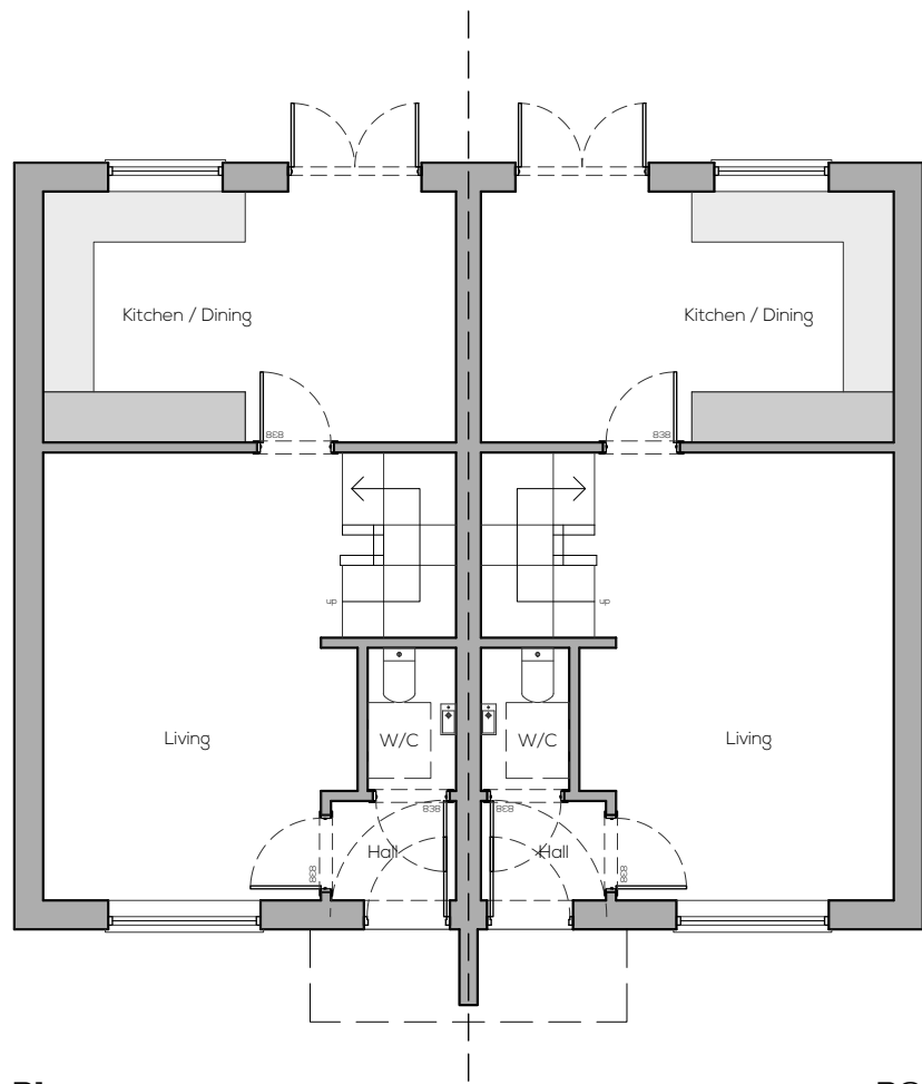
P1 Ground Floor Plans
