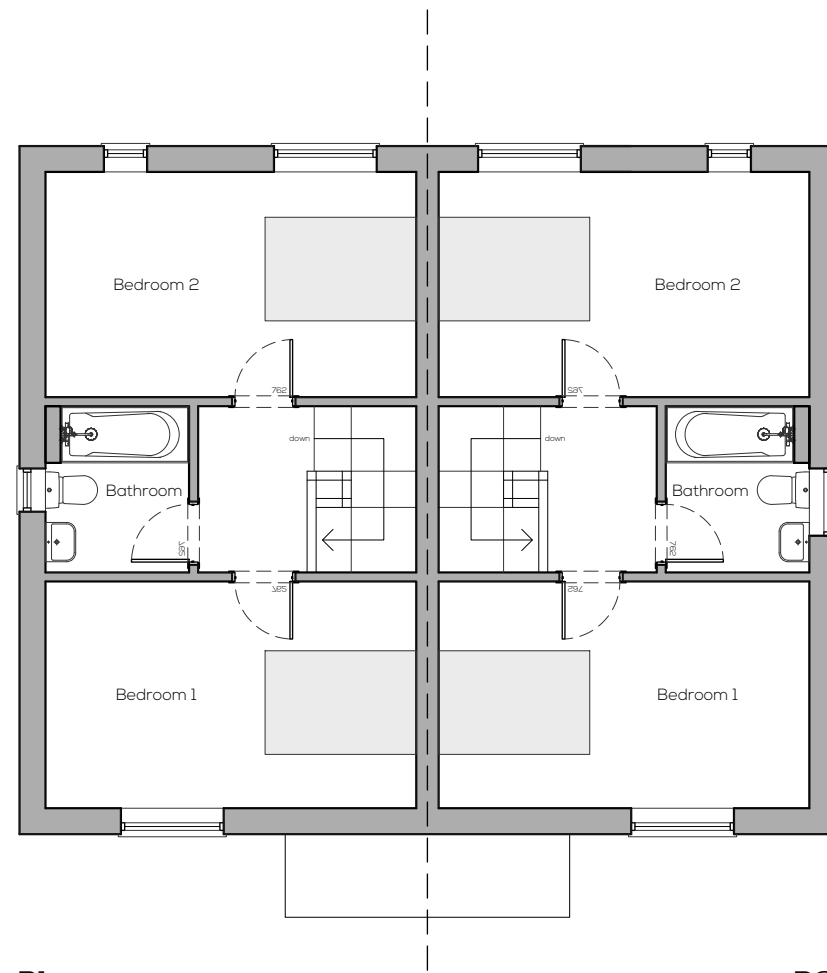
P1 First Floor Plans
